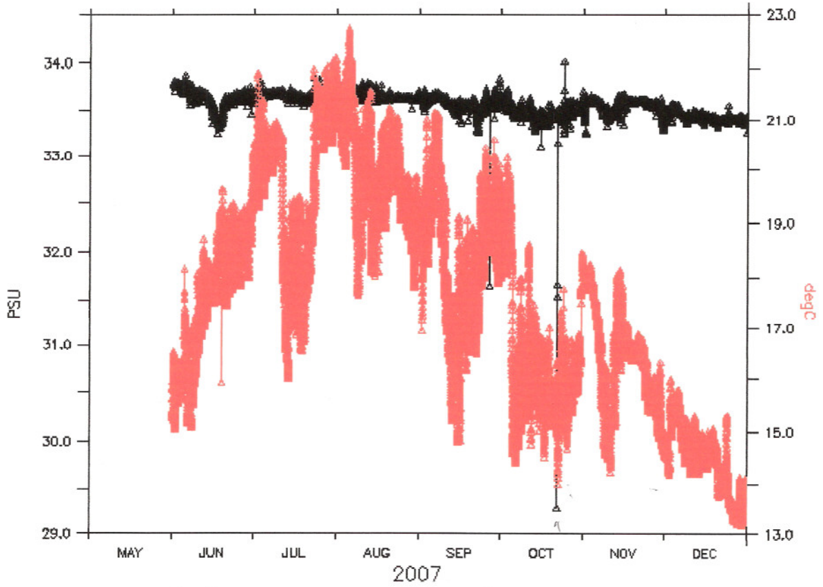
Salinity (PSU) from Santa Monica Bay mooring (CTD: 2007-08 deployment)(1), Temperature (degC) from Santa Monica Bay mooring (CTD: 2007-08 deployment)(2)
