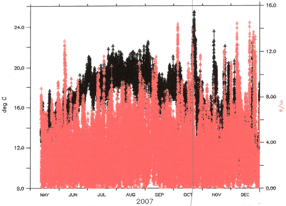
Air temperature (deg C) from Santa Monica Bay mooring (MetSys: 2007-08 deployment)(1), Wind speed (m/s) from Santa Monica Bay mooring (MetSys: 2007-08 deployment)(2)
